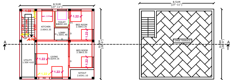
FLOOR - TERRACE PRO. TERRACE FLOOR PLAN
