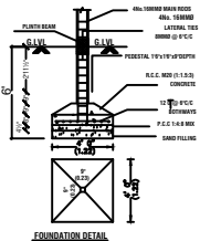
FOUNDATION DETAIL
