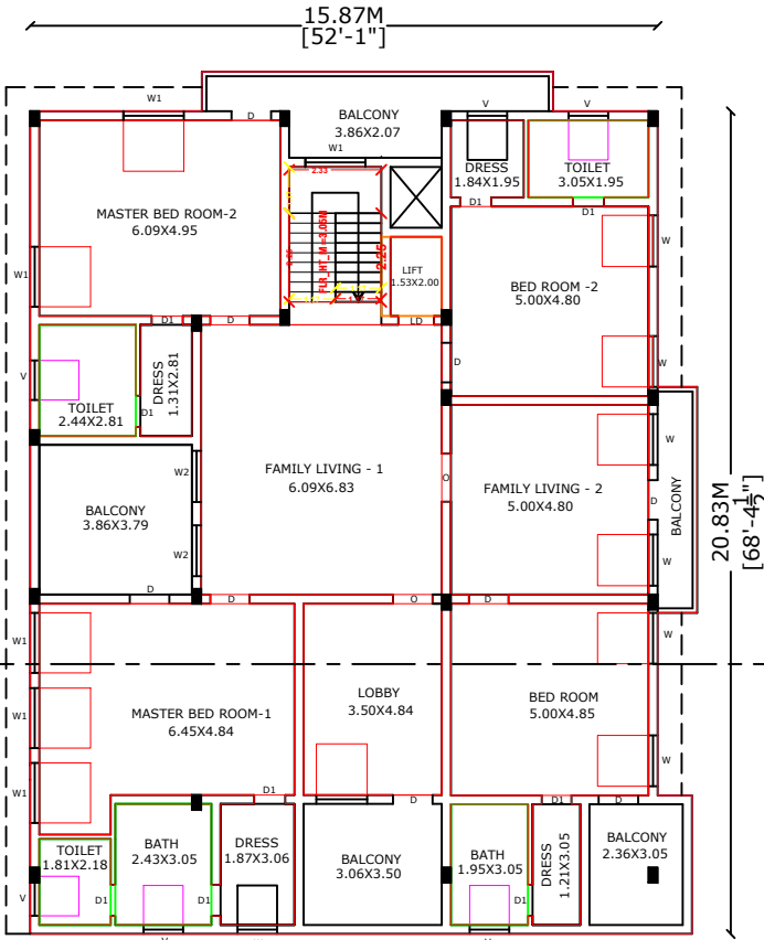
FLOOR - FIRST PRO. FIRST FLOOR PLAN
