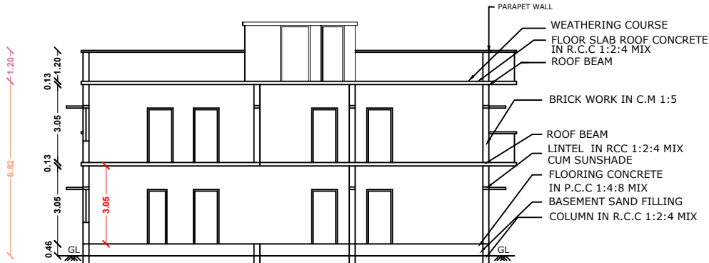
CROSS SECTION ON "A-A"
