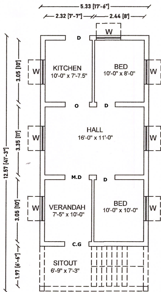
FLOOR PLAN - GROUND [PROPOSED]
