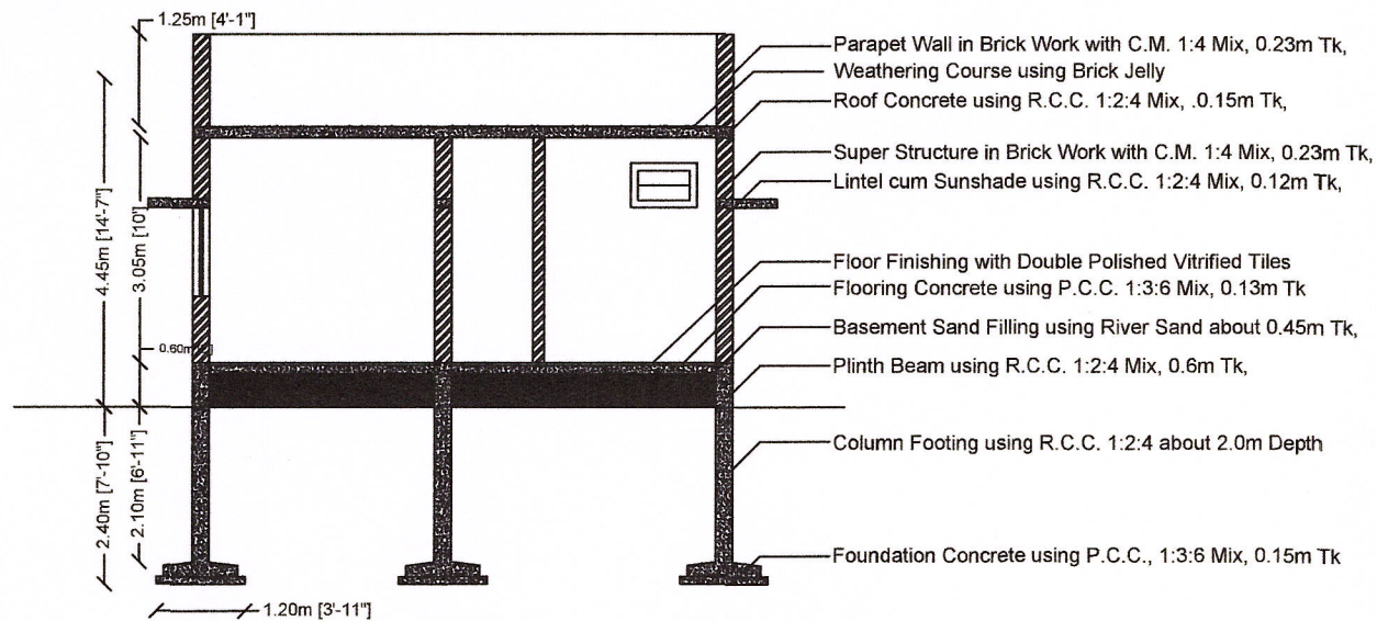
SECTIONAL VIEW ON A-A'
