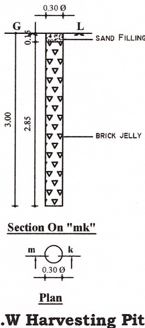
R.W Harvesting Pit
