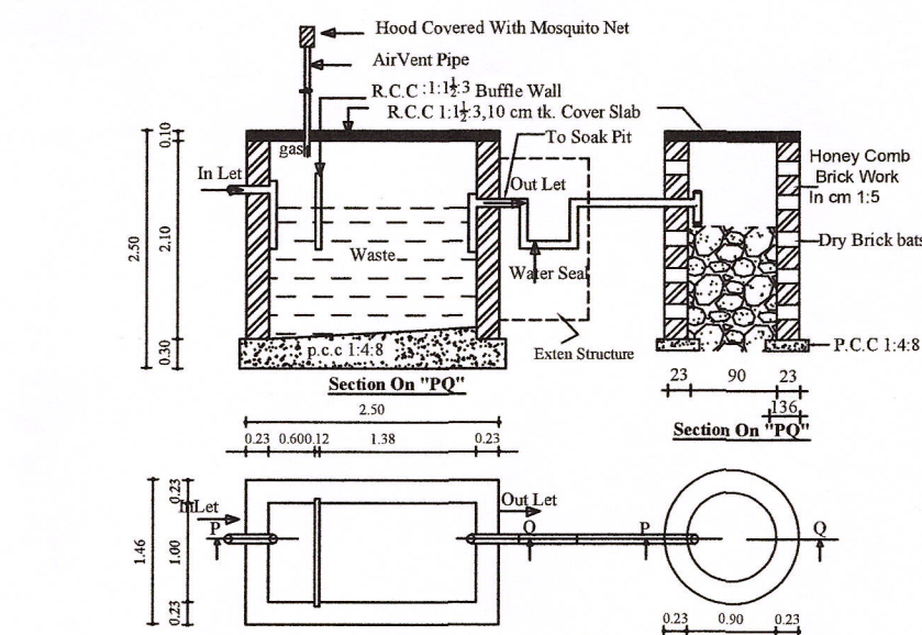
Septic Tank Details Soak Pit Details (SCALE-1:50)
