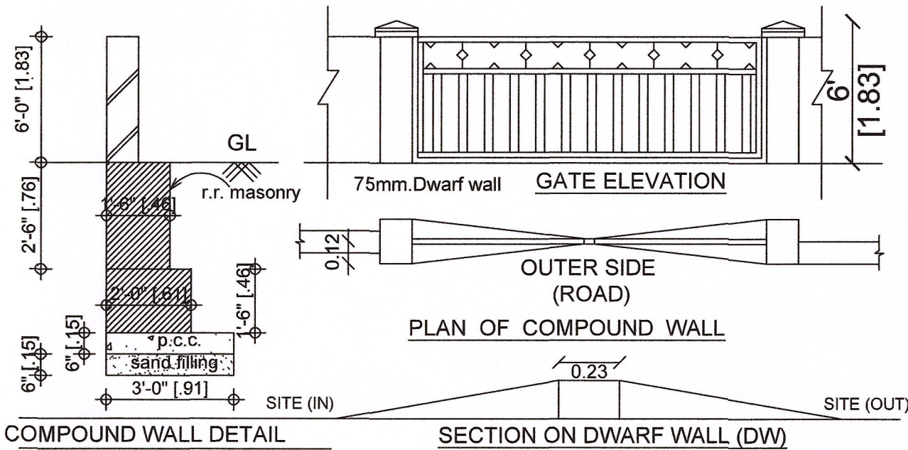
COMPOUND WALL DETAIL
