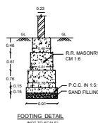
FOOTING DETAIL (NOT TO SCALE)
