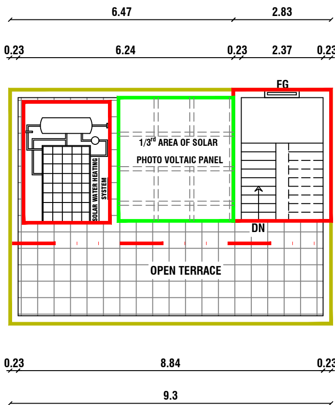
FLOOR - TERRACE
