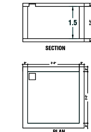
DETAILS OF COLLECTION SUMP FOR RAIN WATER HARVESTING OF ROOF TOP RAIN WATER RW_H_CAPACITY_L=1000LTRS
