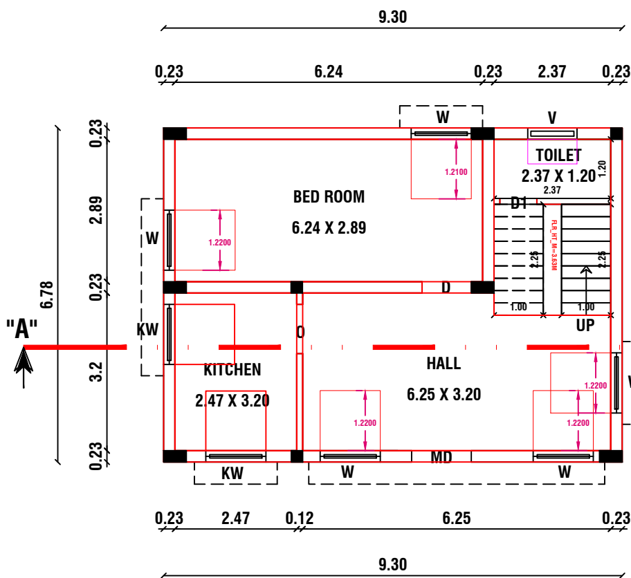
FLOOR - GROUND
