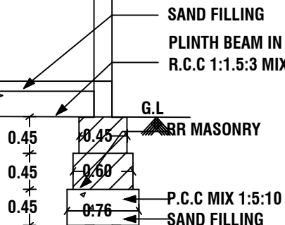
RR MASONRY DETAILS
