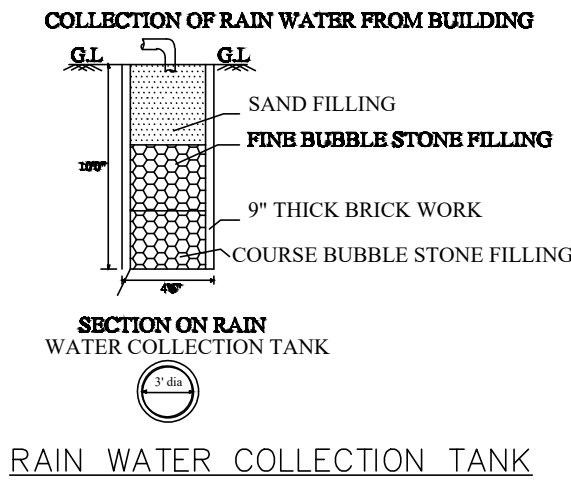
RAIN WATER COLLECTION TANK
