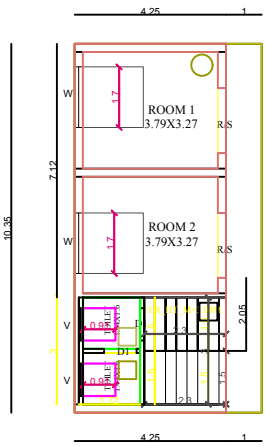
PRO.GROUND FLOOR (G.F) PLAN
