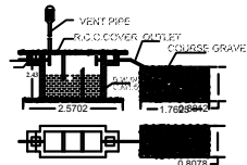
SEPTIC TANK & D-TRENCH DETAILS NOT TO SCALE
