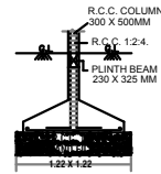
FOUNDATION DETAIL (NOT TO SCALE)
