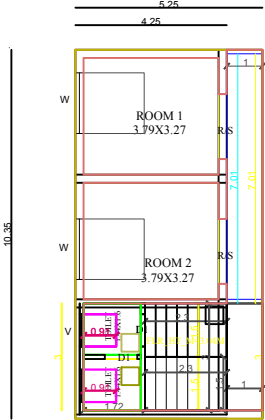
PRO.FIRST FLOOR (F.F) PLAN
