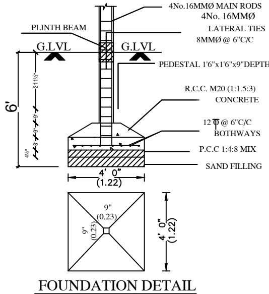
FOUNDATION DETAIL
