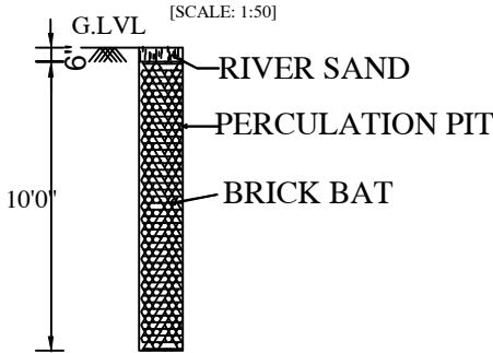
PERCOLATION PIT
