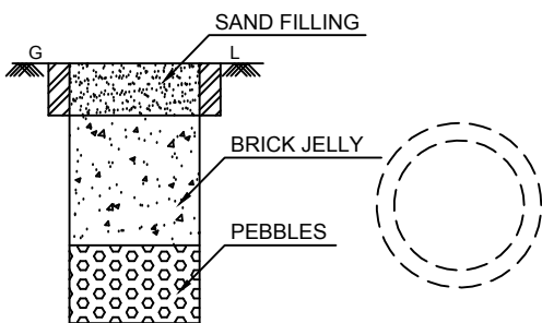
RAIN WATER HARVESTING SYSTEM SCALE 1:50
