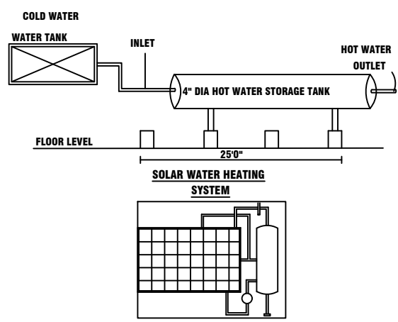
SOLAR HOT WATER SYSTEM DETAILS
