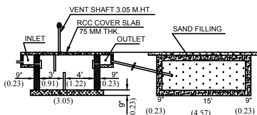
SECTION ON SEPTIC TANK & DISP-TRENCH
