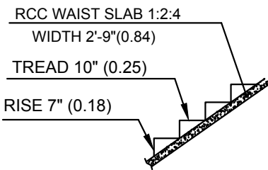
STAIRCASE DETAIL SCALE 1:50
