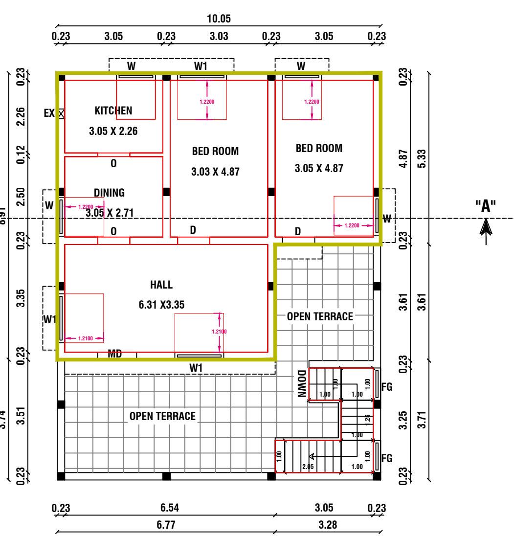
FLOOR - FIRST & TERRACE PRO. FIRST FLOOR PLAN
