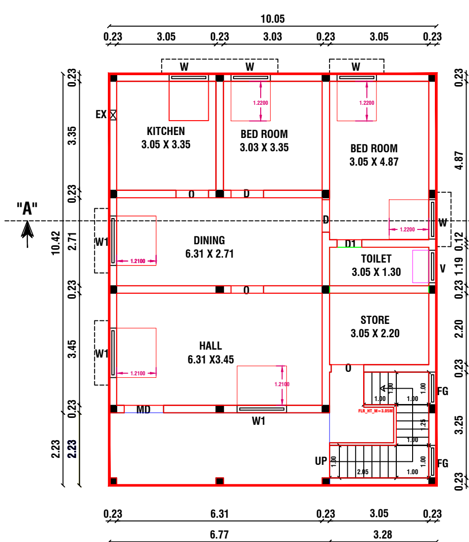
FLOOR - GROUND PRO. GROUND FLOOR PLAN
