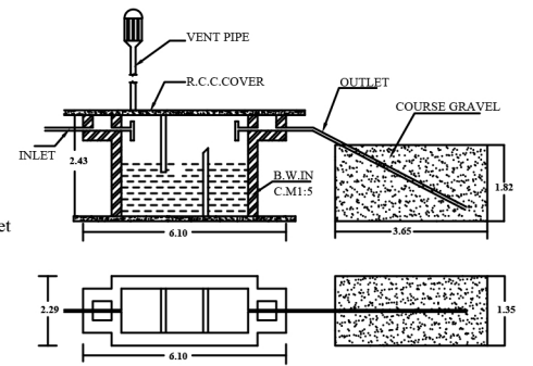
SEPTIC TANK & D-TRENCH DETAILS
