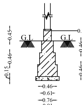
FOOTING DETAILS
