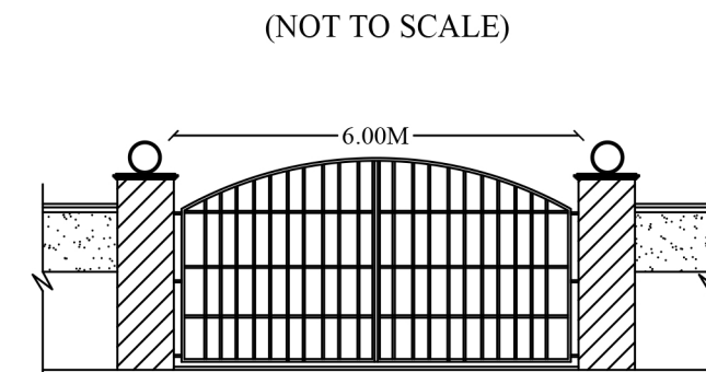
COMPOUND GATE
