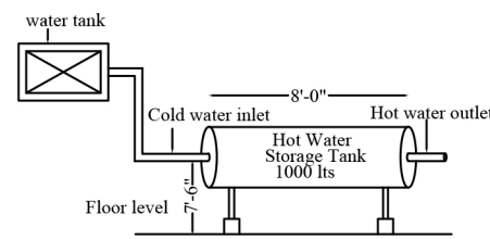
SOLAR WATER HEATER DETAILS
