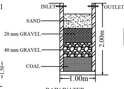
RAIN WATER COLLECTION TANK
