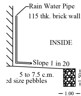
WATER HARVESTING
