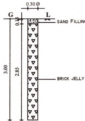
Section On "mk"
