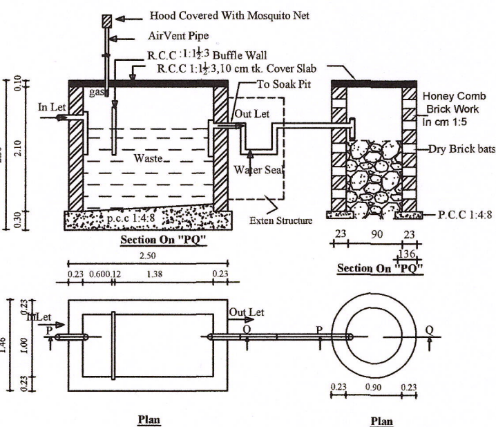
Septic Tank Details Soak Pit Details (SCALE:1:50)
