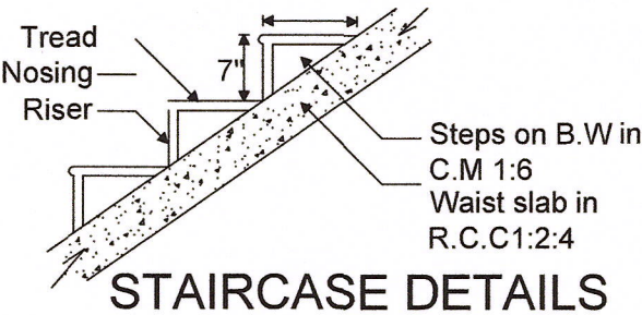
STAIRCASE DETAILS
