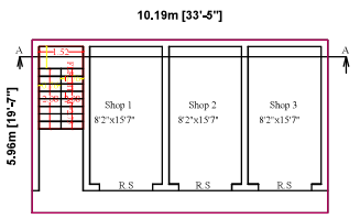
EXG.GROUND FLOOR PLAN
