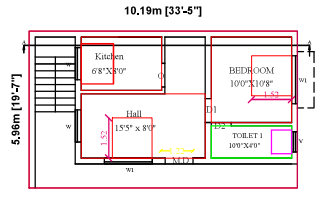
PRO.FIRST FLOOR PLAN
