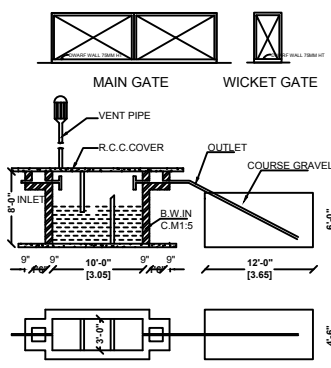
SEPTIC TANK & D-TRENCH DETAILS (NOT TO SCALE)
