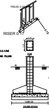
STAIRCASE DETAILS (NOT TO SCALE)
