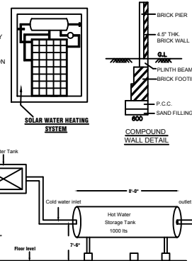
SOLAR WATER HEATER DETAILS
