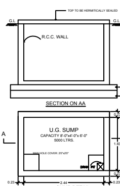
SUMP DETAIL
