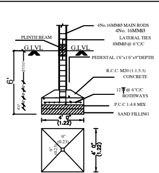
FOUNDATION DETAIL
