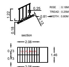
STAIRCASE DETAIL
