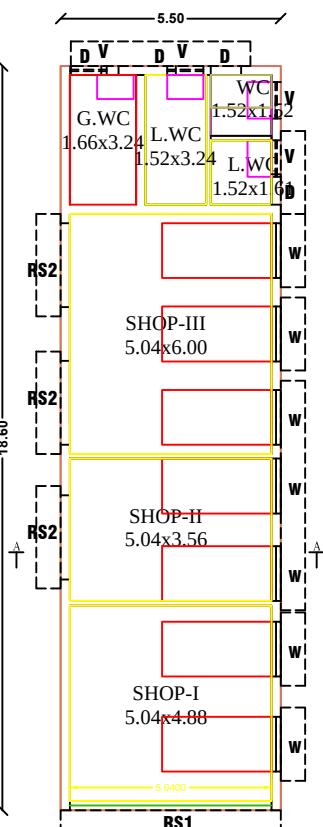
FLOOR-GROUND PROPOSED GROUND FLOOR PLAN COMMERCIAL SHOPS
