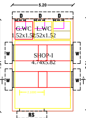
FLOOR-GROUND PROPOSED GROUND FLOOR PLAN COMMERCIAL SHOPS
