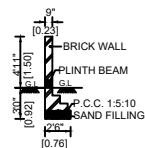
SECTION - CC
