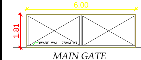
MAIN GATE
