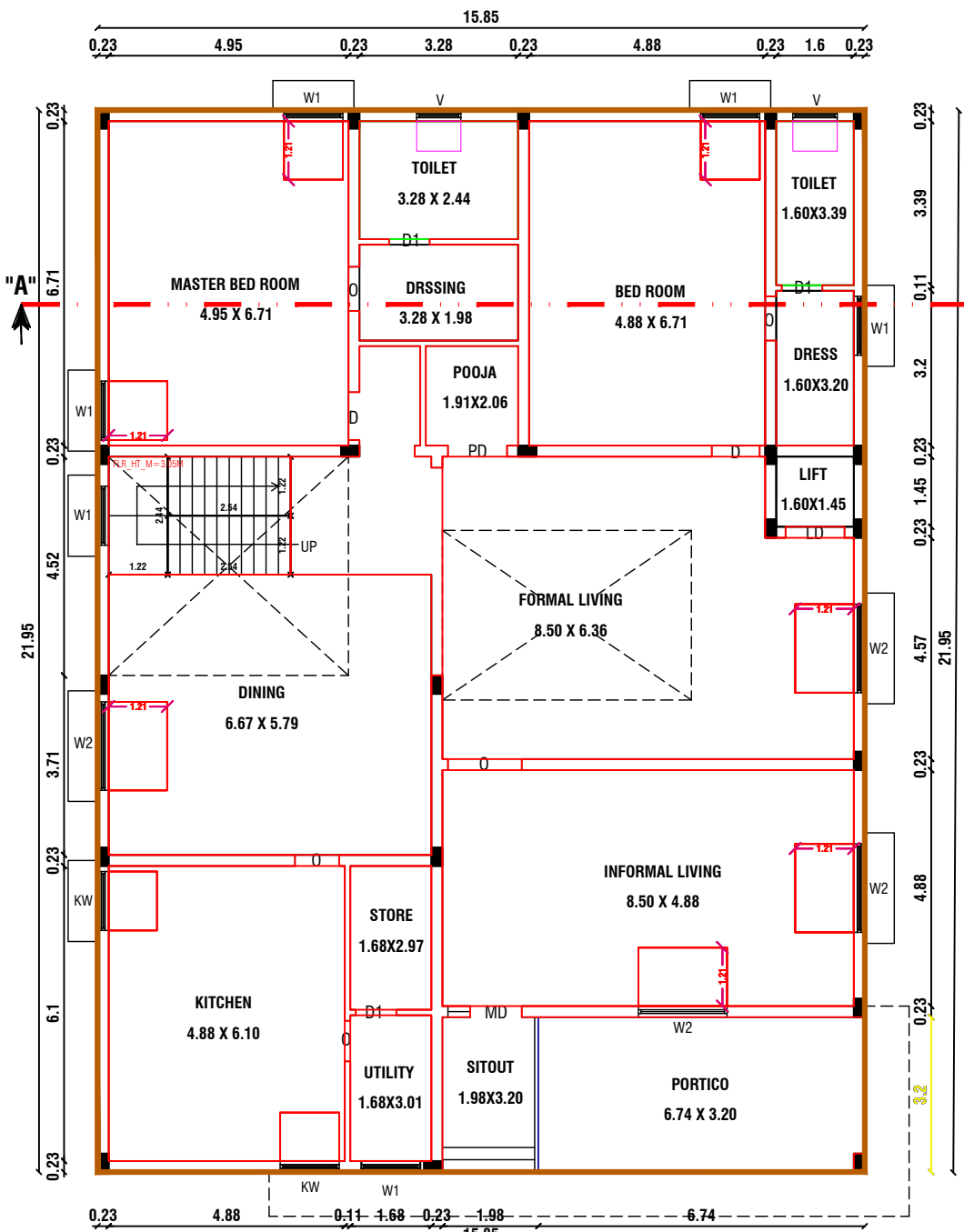
FLOOR - GROUND PRO. GROUND FLOOR PLAN
