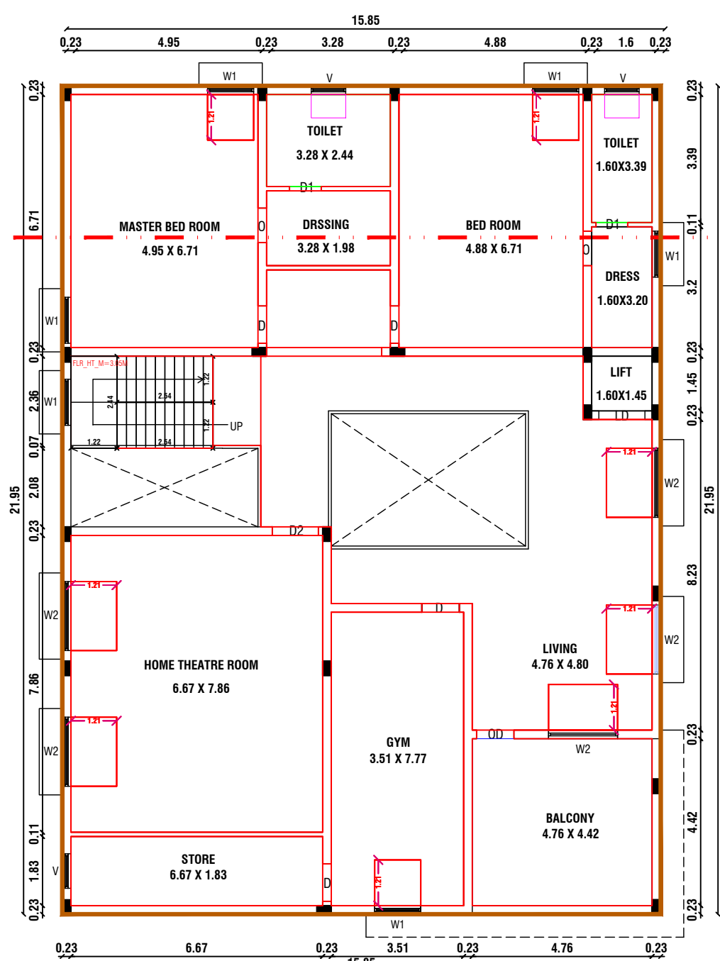
FLOOR - FIRST PRO. FIRST FLOOR PLAN
