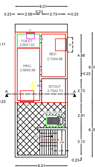
PRO.SECOND FLOOR PLAN
