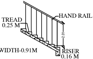
STAIRCASE DETAILS
