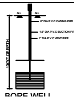
ROPE WELL
