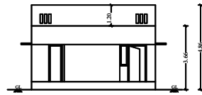
FRONT ELEVATION
