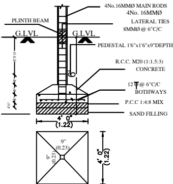
FOUNDATION DETAIL
