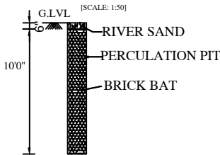
PERCOLATION PIT
