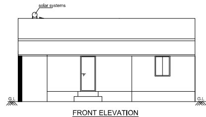
DETAILED PLAN: SCALE 1:100
