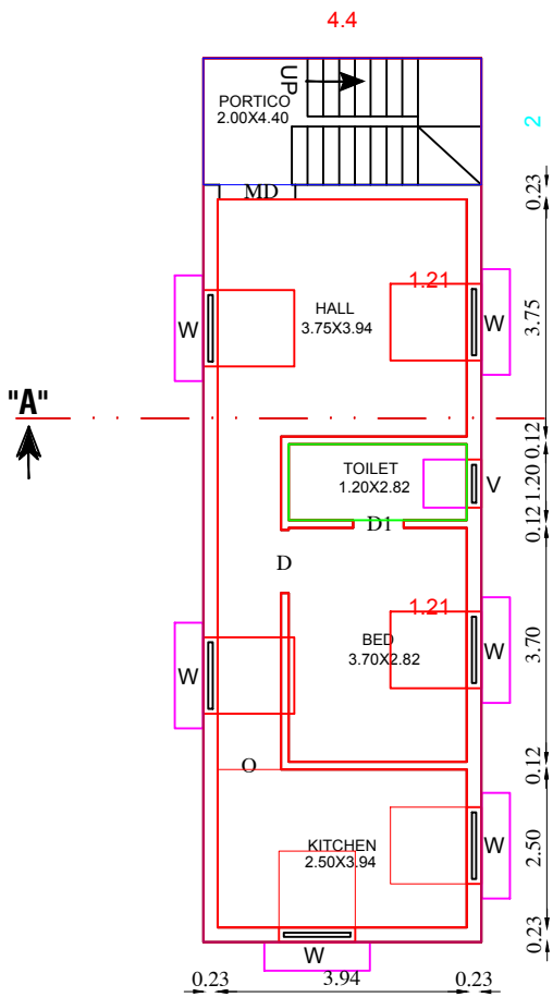
FLOOR - GROUND
