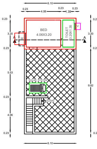
PROPOSED SECOND FLOOR PLAN
