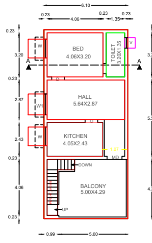
PROPOSED FIRST FLOOR PLAN
