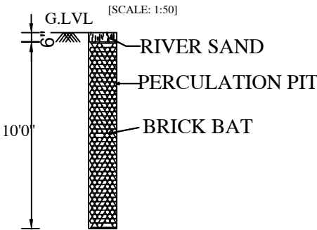
PERCULATION PIT
