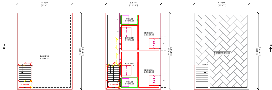
FLOOR - GROUND PRO. GROUND FLOOR PLAN
