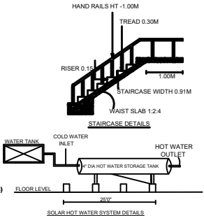
SOLAR HOT WATER SYSTEM DETAILS
