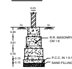
FOOTING DETAIL NOT TO SCALE
