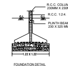
FOUNDATION DETAIL NOT TO SCALE
