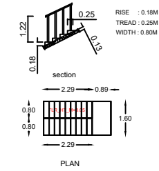
STAIRCASE DETAIL
