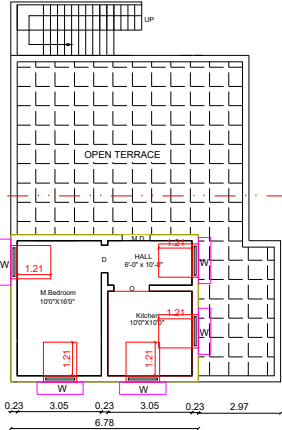
FLOOR - FIRST
