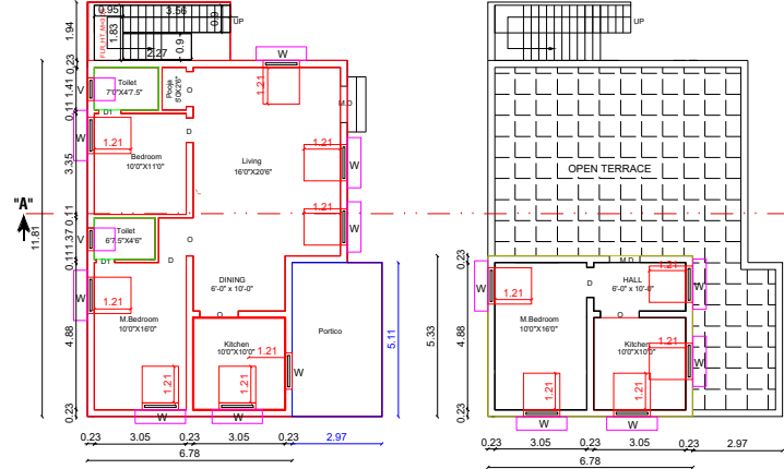
FLOOR - GROUND
