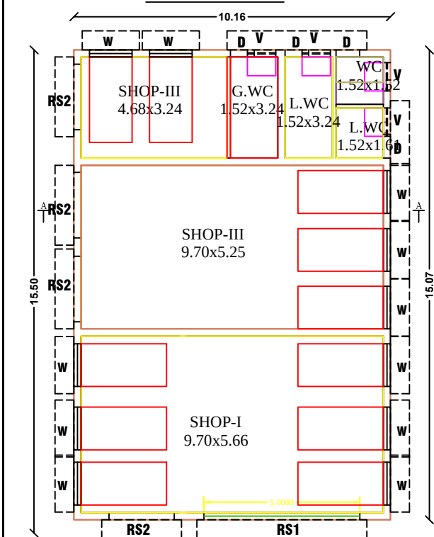
FLOOR-GROUND PROPOSED GROUND FLOOR PLAN COMMERCIAL SHOPS
