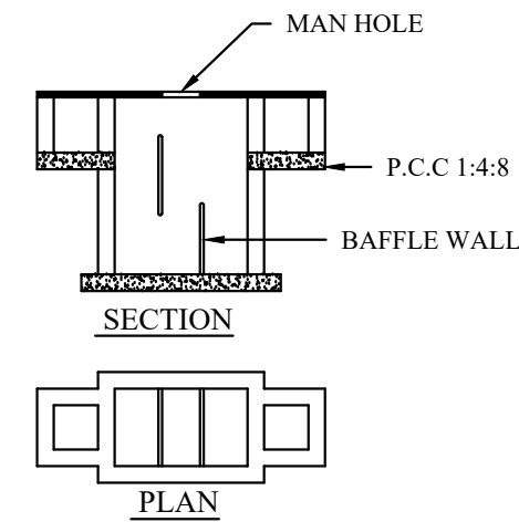
SEPTIC-TANK DETAIL
