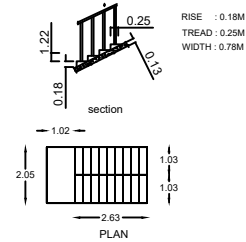
STAIRCASE DETAIL
