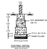
FOOTING DETAIL (NOT TO SCALE)
