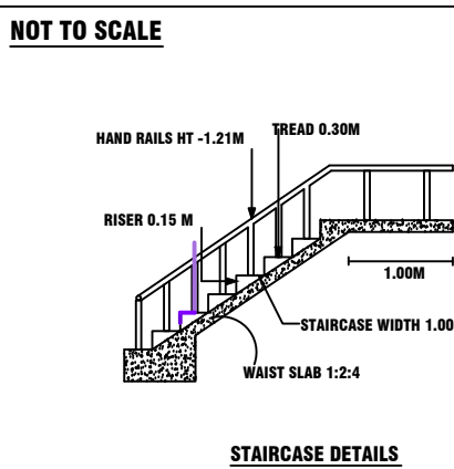
STAIRCASE DETAILS
