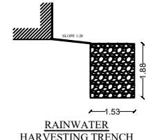
RAINWATER HARVESTING TRENCH
