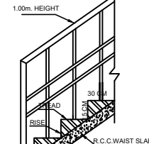
SECTION ON STAIRCASE
