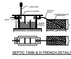
SEPTIC TANK & D-TRENCH DETAILS
