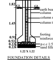
FOUNDATION DETAILS
