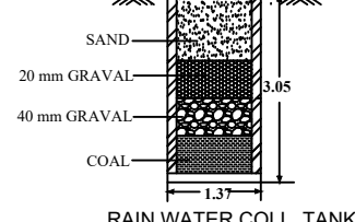
RAIN WATER COLL .TANK (NTS)
