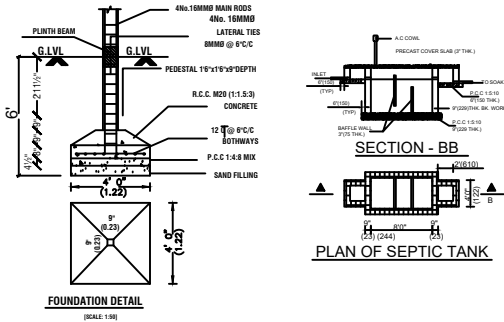
FOUNDATION DETAIL
