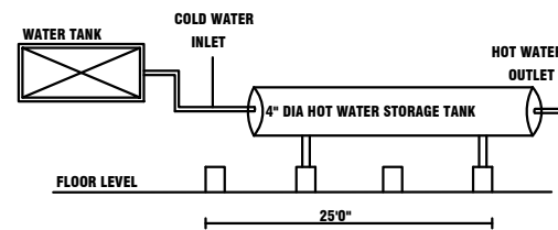
SOLAR HOT WATER SYSTEM DETAILS
