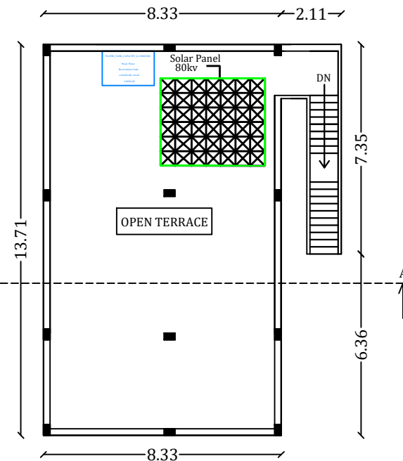
PRO.TERRACE FLOOR PLAN
