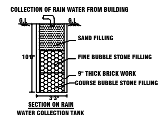
WATER COLLECTION TANK
