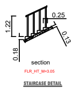
STAIRCASE DETAIL (NOT TO SCALE)
