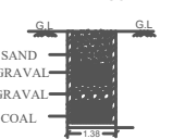
SECTION NO RAIN WATER COLL. TANK
