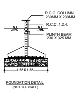
FOUNDATION DETAIL (NOT TO SCALE)
