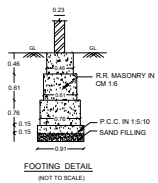
FOOTING DETAIL (NOT TO SCALE)
