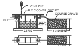
SEPTIC TANK & D-TRENCH DETAILS
