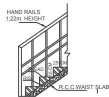
SECTION ON STAIRCASE
