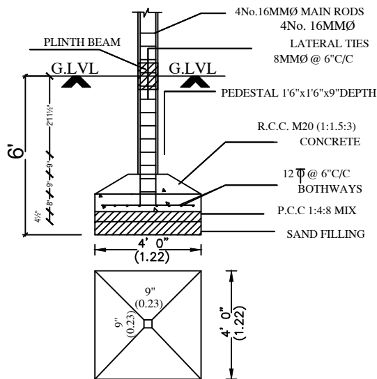
FOUNDATION DETAIL
