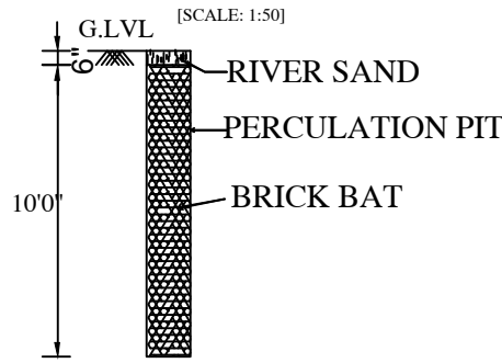
PERCOLATION PIT
