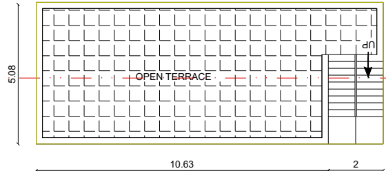
FLOOR - TERRACE PRO.TERRACE FLOOR PLAN
