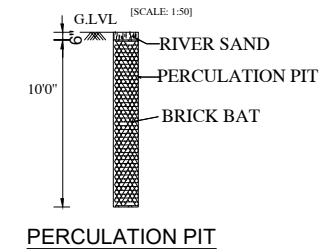
PERCOLATION PIT
