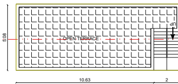
FLOOR - TERRACE PRO.TERRACE FLOOR PLAN
