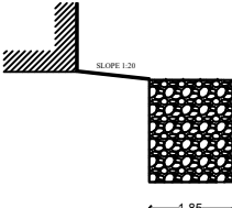
RAINWATER HARVESTING TRENCH
