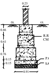
FOOTING DETAIL
