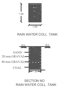
RAIN WATER COLL. TANK
