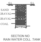
SECTION NO RAIN WATER COLL. TANK
