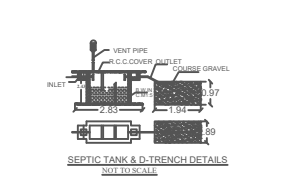
SEPTIC TANK & D-TRENCH DETAILS NOT TO SCALE
