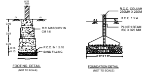
FOOTING DETAIL NOT TO SCALE
