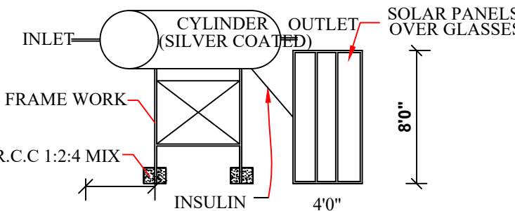
WASTE WATER RECYCLE UNIT
